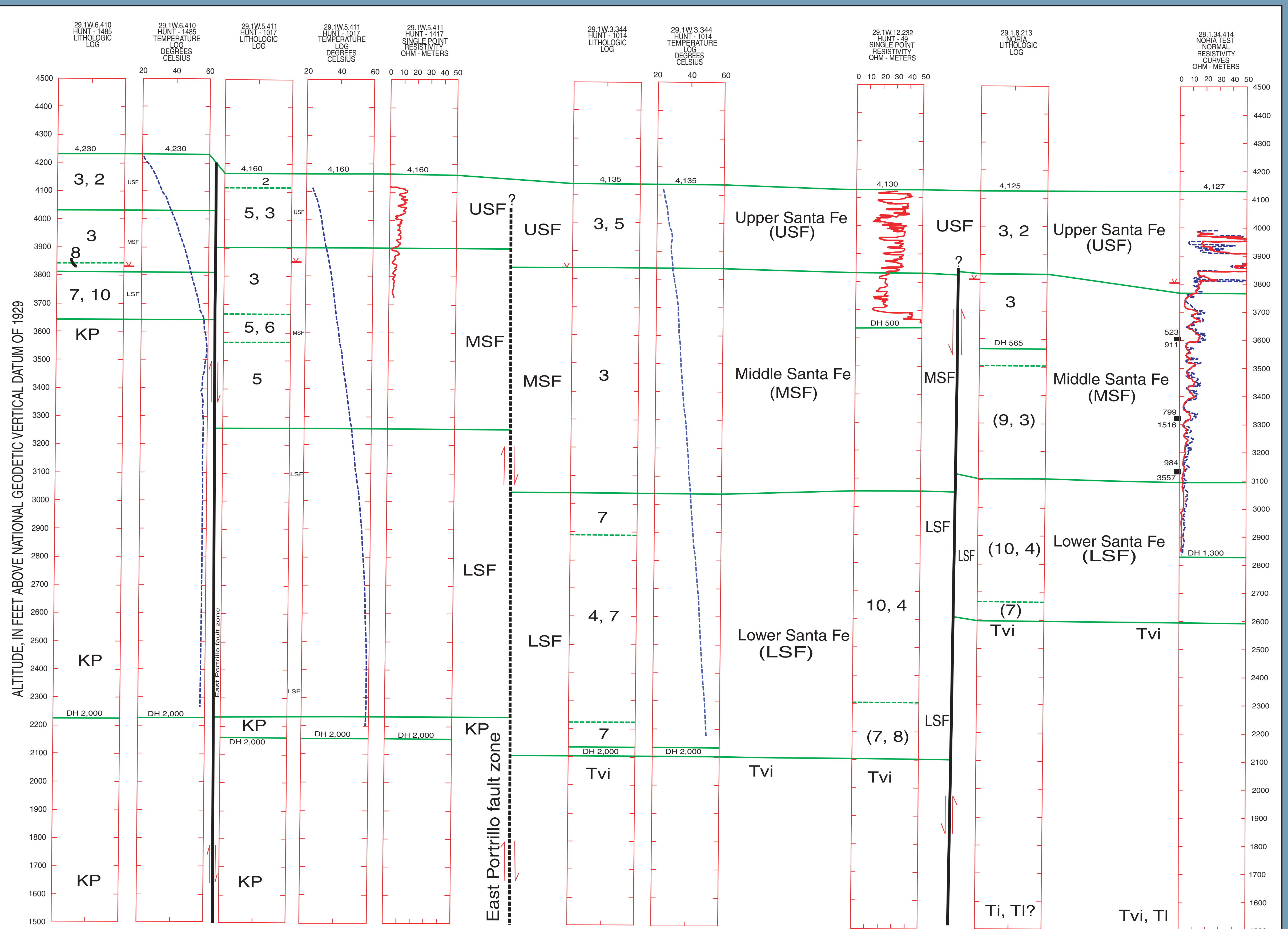
Plate 4w. Hydrogeologic section Potrillo Mountains to Noria Test, with borehole geophysical data.
