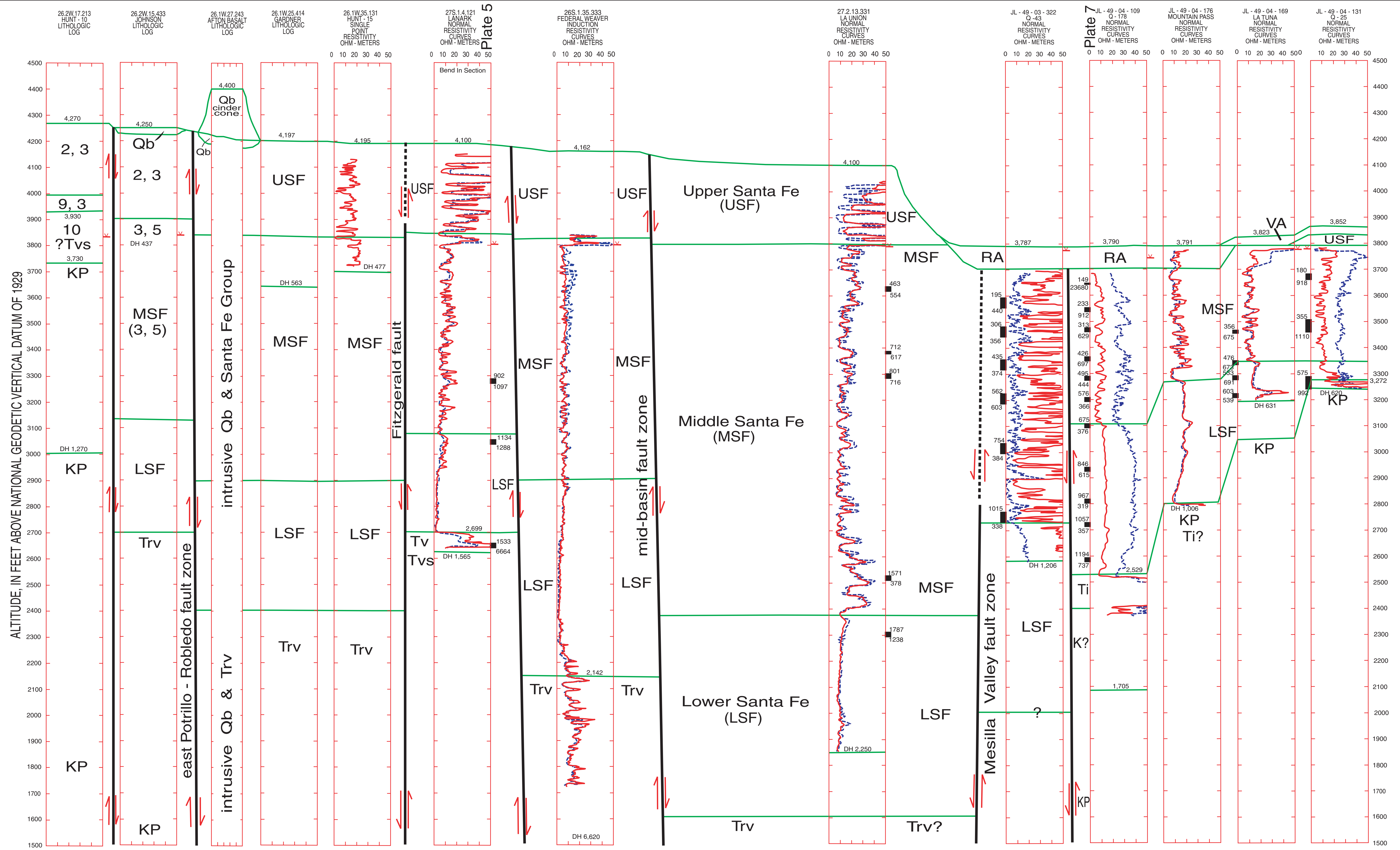
Plate 3. Hydrogeologic section Aden to La Tuna, with borehole geophysical data.
