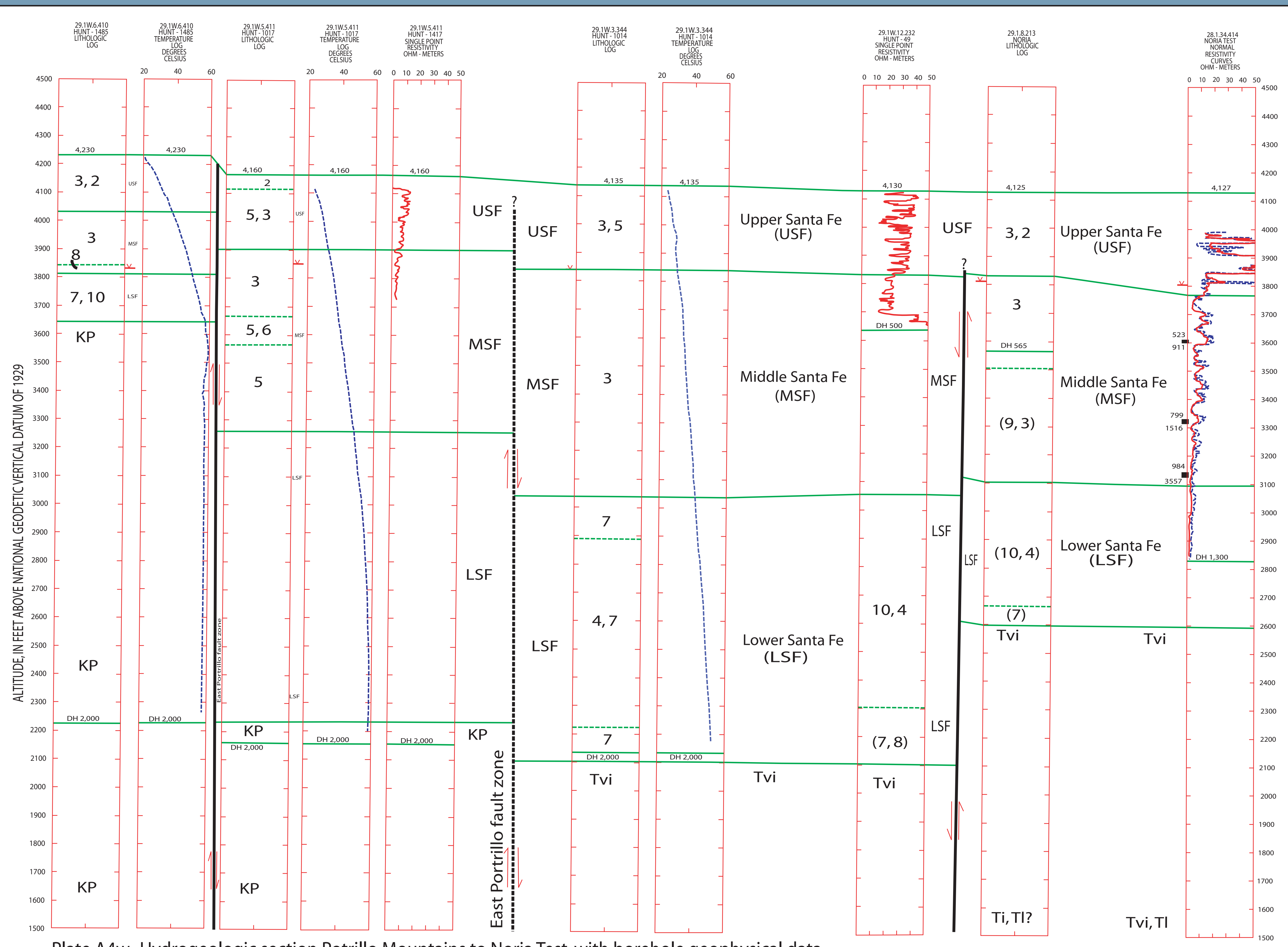
Plate A4w. Hydrogeologic section Potrillo Mountains to Noria Test, with borehole geophysical data.
