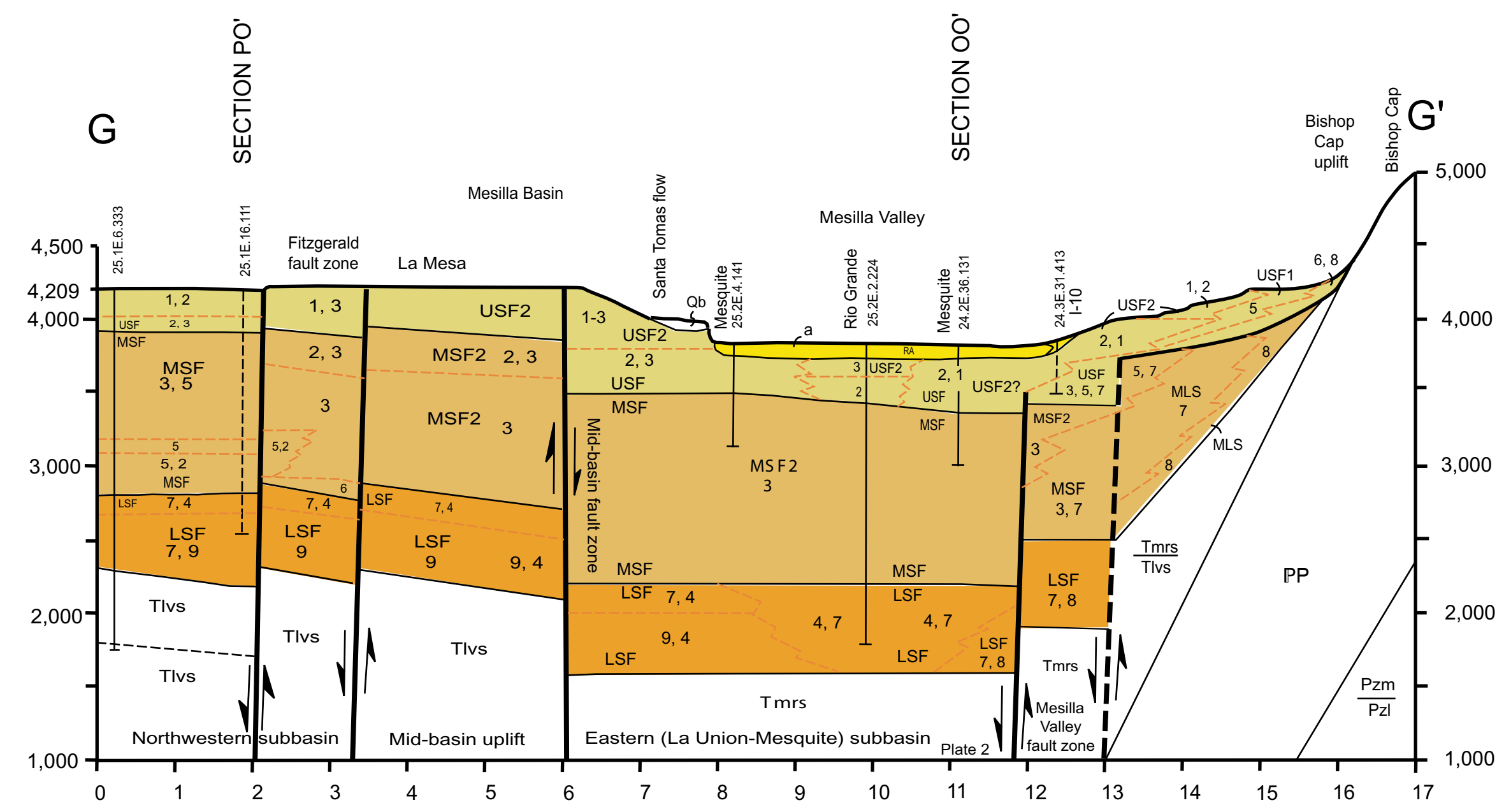
4a. Section G-G' - Eastern Mesilla Basin and Valley: West Mesa and Santo Tomas volcanic center to Bishop Cap uplift.
