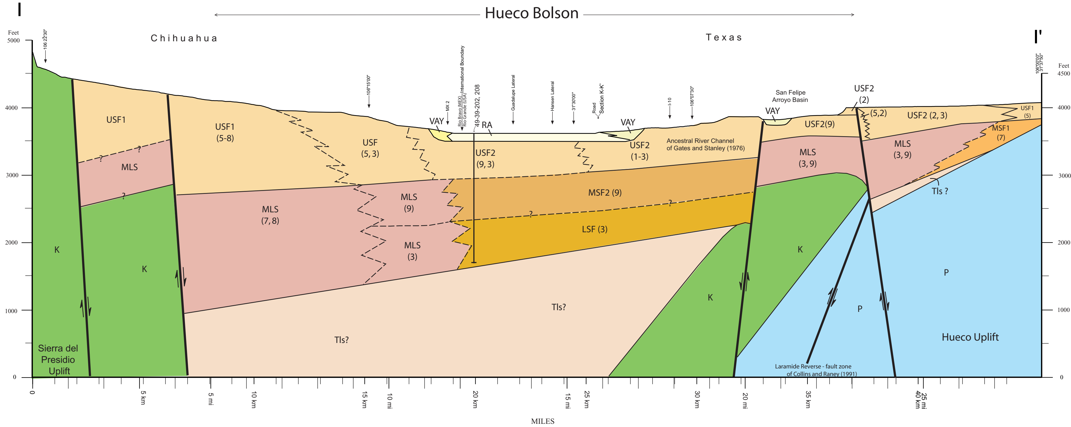
Schematic Hydrogeologic Section -- I-I' - from Sierra del Presidio to Hueco uplift, across Fabens area of west-central Hueco Bolson
