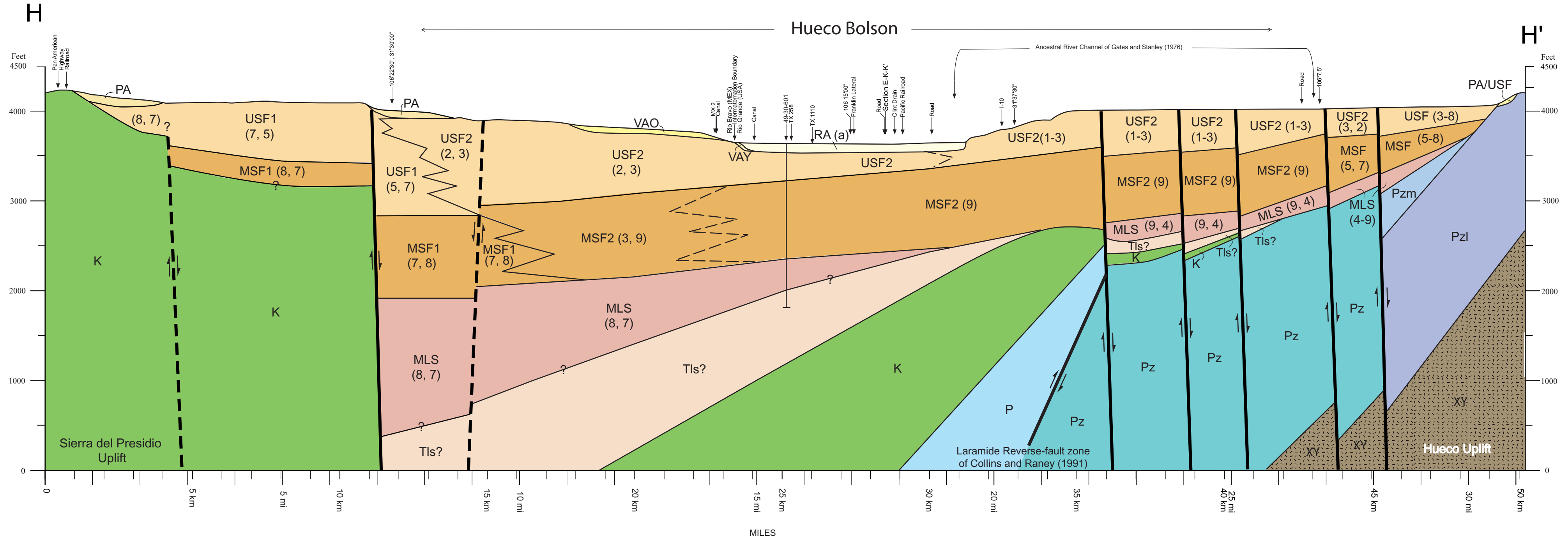
Schematic Hydrogeologic Section -- H-H' - from western Sierra del Presidio to Hueco uplift, across San Elizario area of southwestern Hueco Bolson
