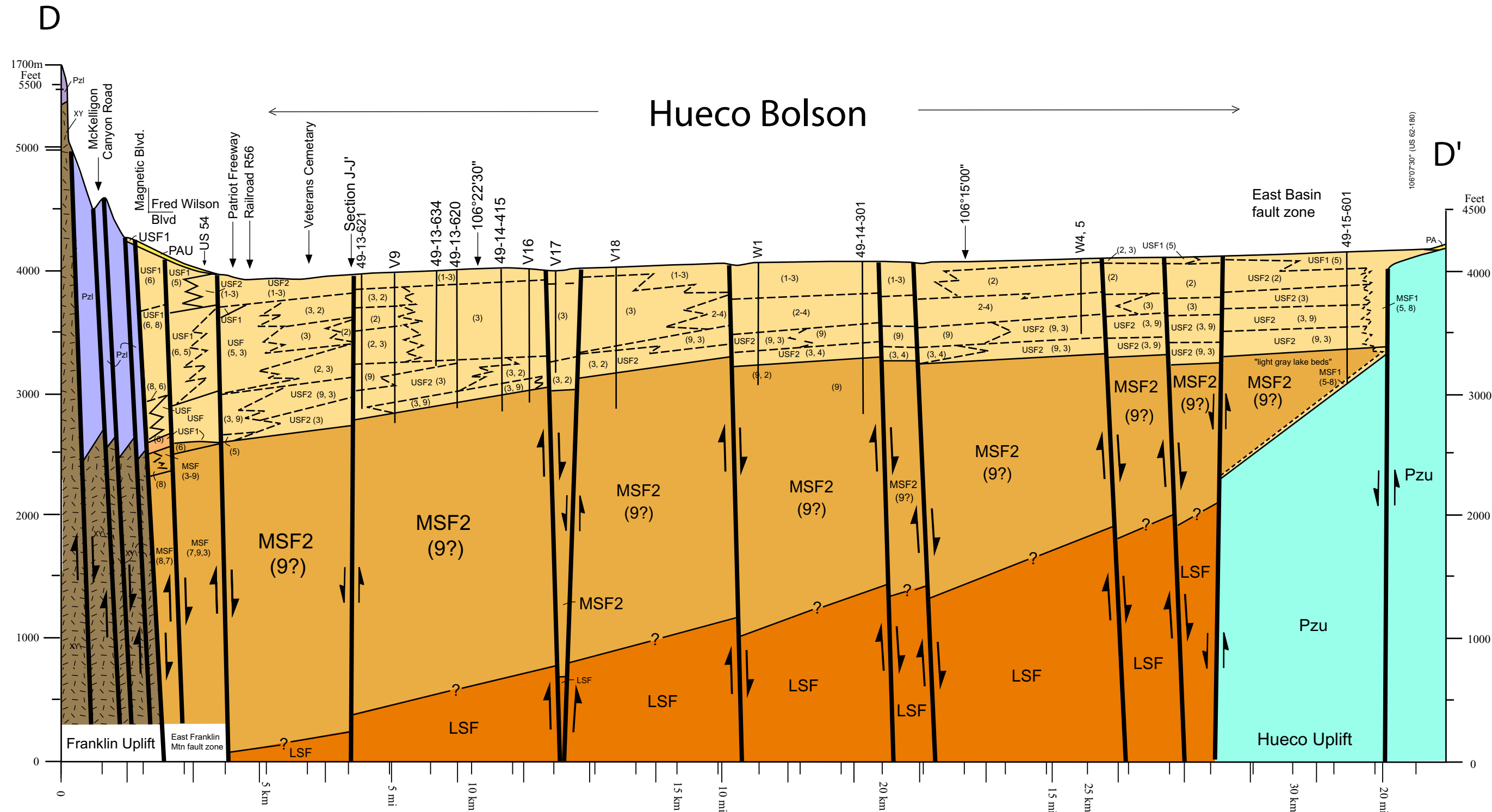
Schematic Hydrogeologic Section -- D-D' - from southern Franklin Mountains-McKelligon Canyon to Hueco uplift, across Fort Bliss area of north-central Hueco Bolson-Fred Wilson Road alignment
