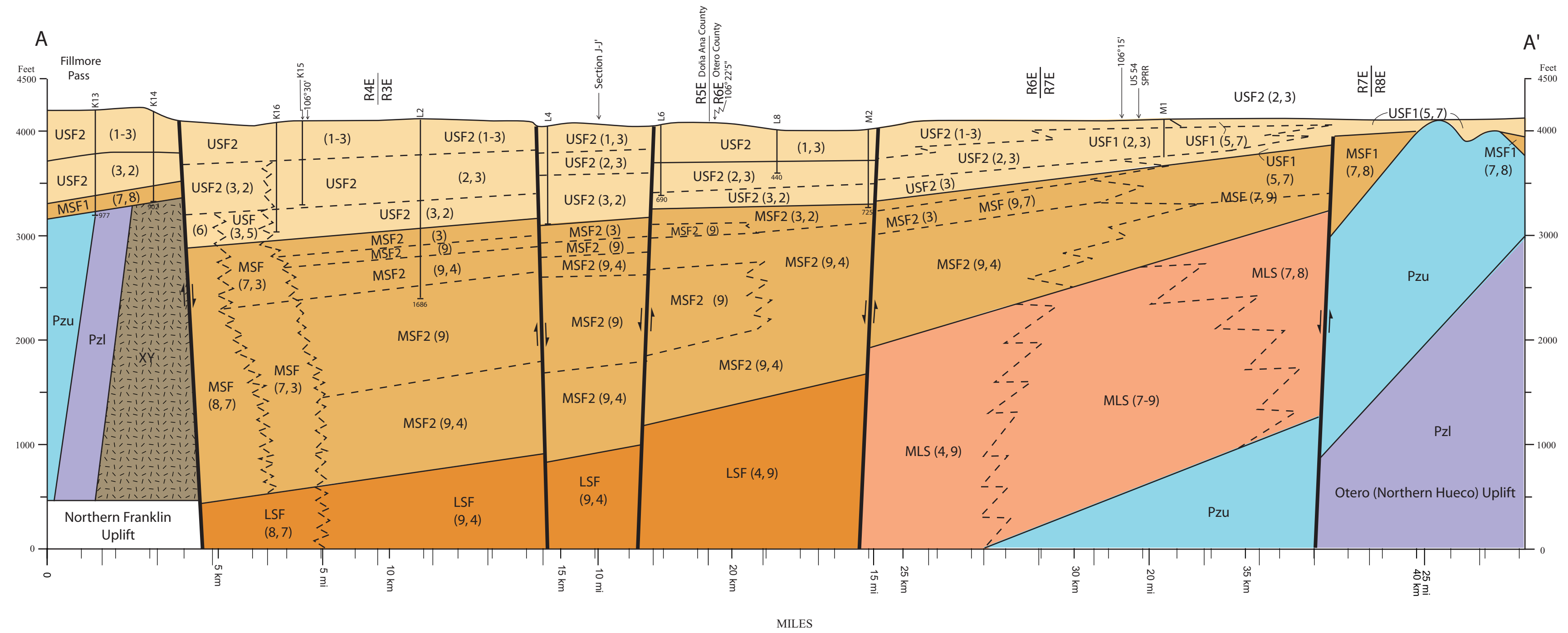
Schematic Hydrogeologic Section -- A-A' - Fillmore Pass to Otero uplift, across Hueco Bolson-Tularosa Basin transition zone, south-central New Mexico
