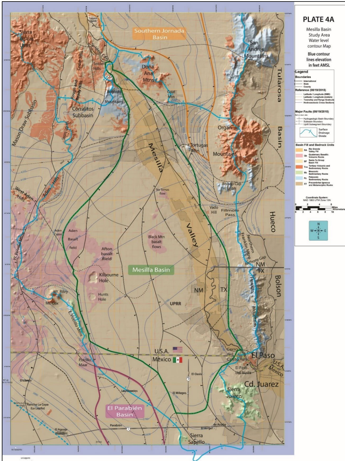
Figure 8-3 (page-size PL. 4A ). Index map for the Study Area’s primary geohydrologic features on a PLATE 1 hydrogeologic-map base. The approximate pre-development (~1976) potentiometric-surface altitude (amsl) is shown with 20- and 100-ft contours. Major surface-watershed divides are shown by solid and dashed thick blue lines. The dashed blue line with arrows in the map’s SW corner marks the approximate boundary between EPdN- and ZHGCM (El Barreal)-directed GW flow.
