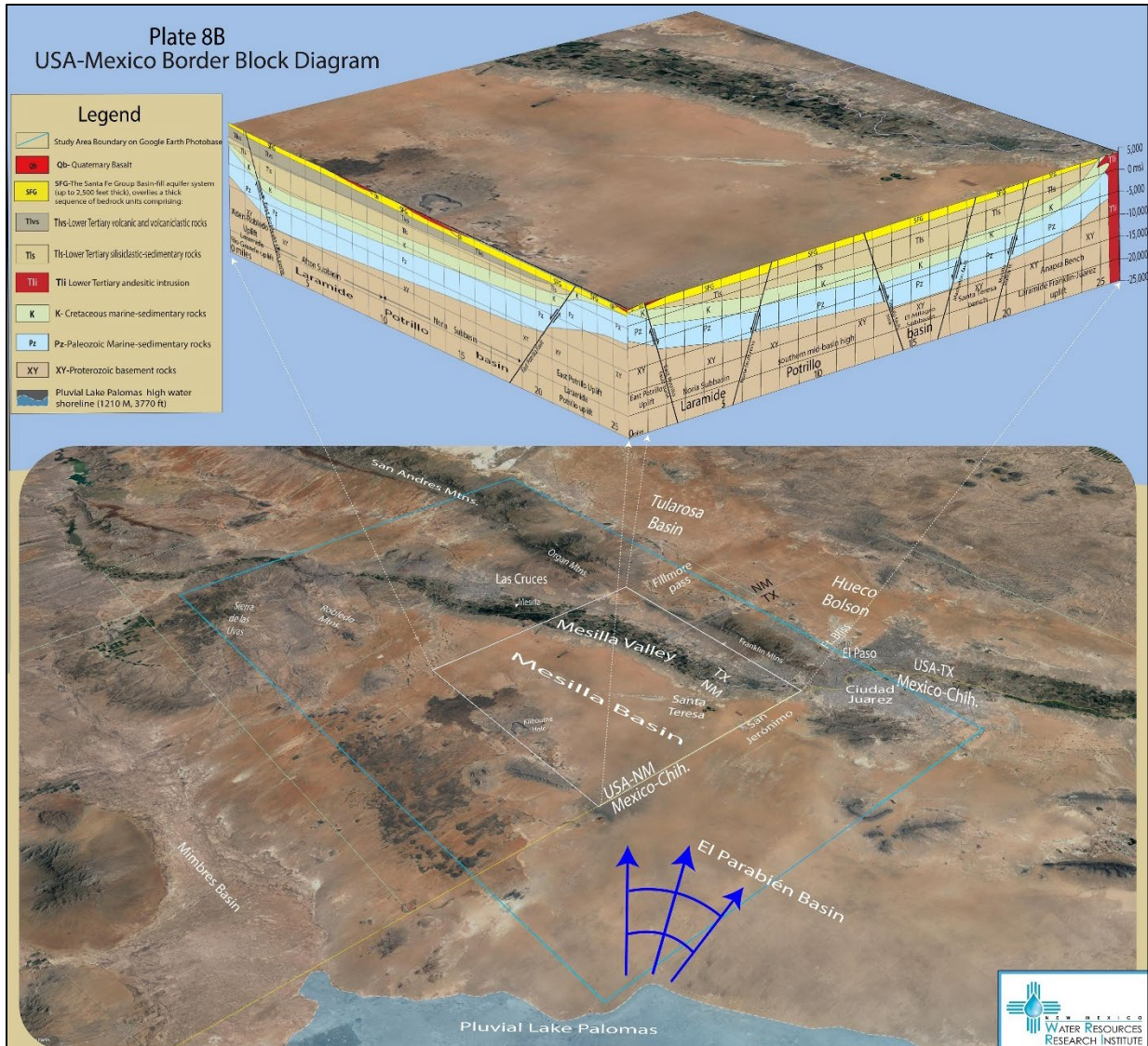
Figure 3-11 (page-size PL. 8B ). Northeast-facing block diagram of the southern Mesilla Basin, with its southern panel at the International-Boundary and stratigraphic-unit definitions on Table 3-1 . It schematically portrays major RG-rift stratigraphic and structural features, including the Eocene Cristo Rey igneous-intrusive complex to a base elevation of 25,000 ft (~7.6 km) below mean sea level (msl). The pale-blue shading at the base of the circular 2017 Google Earth® image show the part of the NE Los Muertos Basin floor that was inundated by Late Pleistocene pluvial-Lake Palomas stands between about 28,000 and 12,000 years ago ( Figs. 1-9 and 1-10 ). Blue arrows show Mesilla Valley-directed outflow component of GW discharge during Lake Palomas high stands (3,940-3,970-ft / 1,201-1,210-m amsl).
