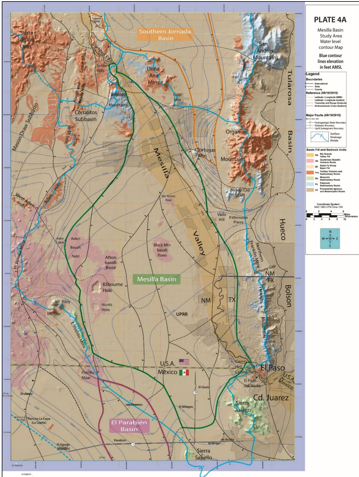
Figure 7-2a (page-size PL. 4A ). Index map for major geohydrologic features of the NM WRI Study Area (~1976 potentiometric-surface altitude in 10 and 100 ft amsl intervals). PLATE 1 Hydrogeologic-Map DEM base.
