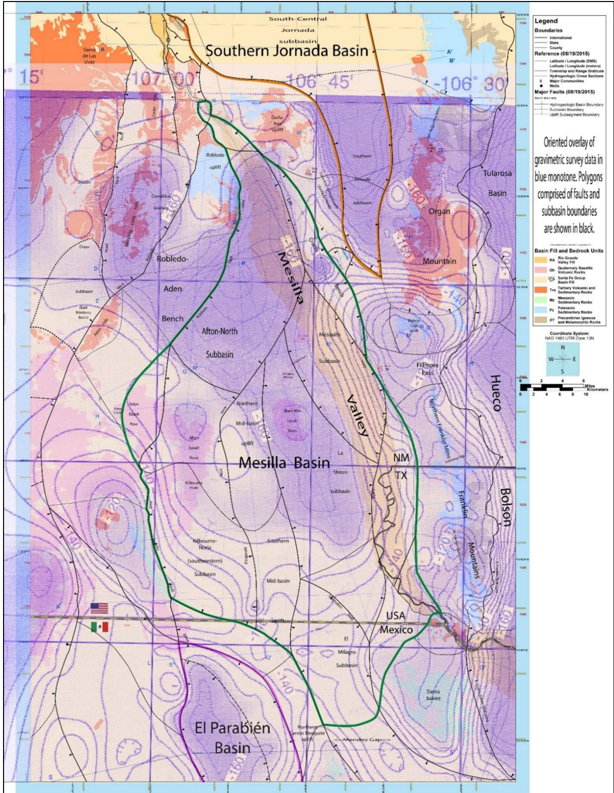
Figure 3-8 (page-size PL. 2A ). Digital overlay of Bouguer isostatic-residual gravity map (4 milligal contour interval) on the Study Area's hydrogeologic-basemap ( Fig. 1-8 [PL. 1B] ). The MeB and parts of the Southern Jornada and El Parabién GW Basins outlined in green, orange and dark red, respectively.
