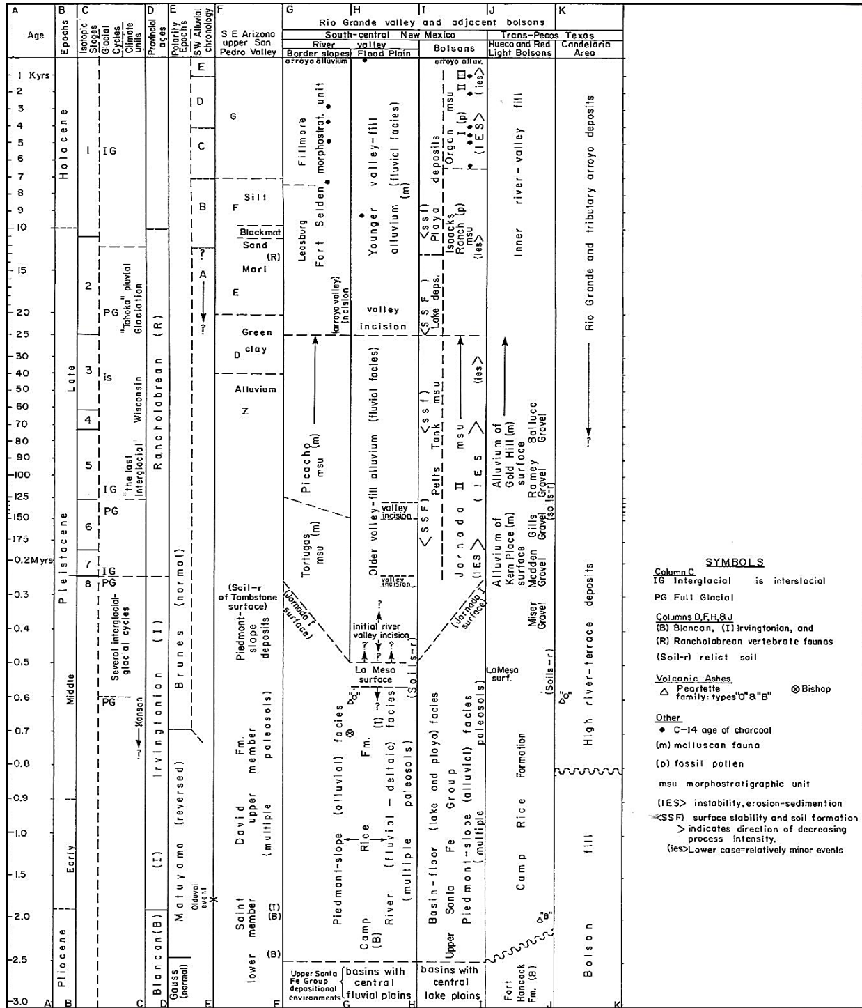
Figure 3-18 (Gile et al. 1981, Fig. 8). Correlation diagram for representative stratigraphic units and geomorphic-process categories of Late Pliocene and Quaternary age in the southern Rio Grande rift region of south-central New Mexico and Trans-Pecos Texas. Adapted from Hawley (1978, Chart 1). A more-detailed explanation for Figure content, including a topical key to Cited References, is in Table 3-4 . See Figure 3-19 for a schematic cross-section view of basic hydrogeologic-framework relationships in the northern Mesilla Valley area.
