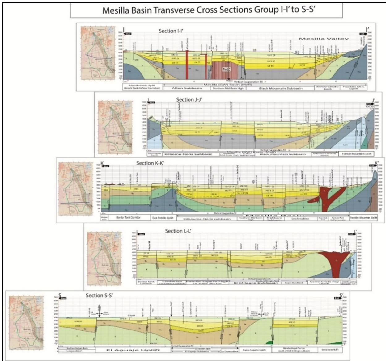
Figure 2-4 (page-size reproduction of PLATE 5i to 5l and 5s panel). Transverse (W to E) hydrogeologic cross-sections I-I' to L-L' and S-S' that span the northern and central parts of the International Boundary Zone (IBZ–Fig. 1-11).
