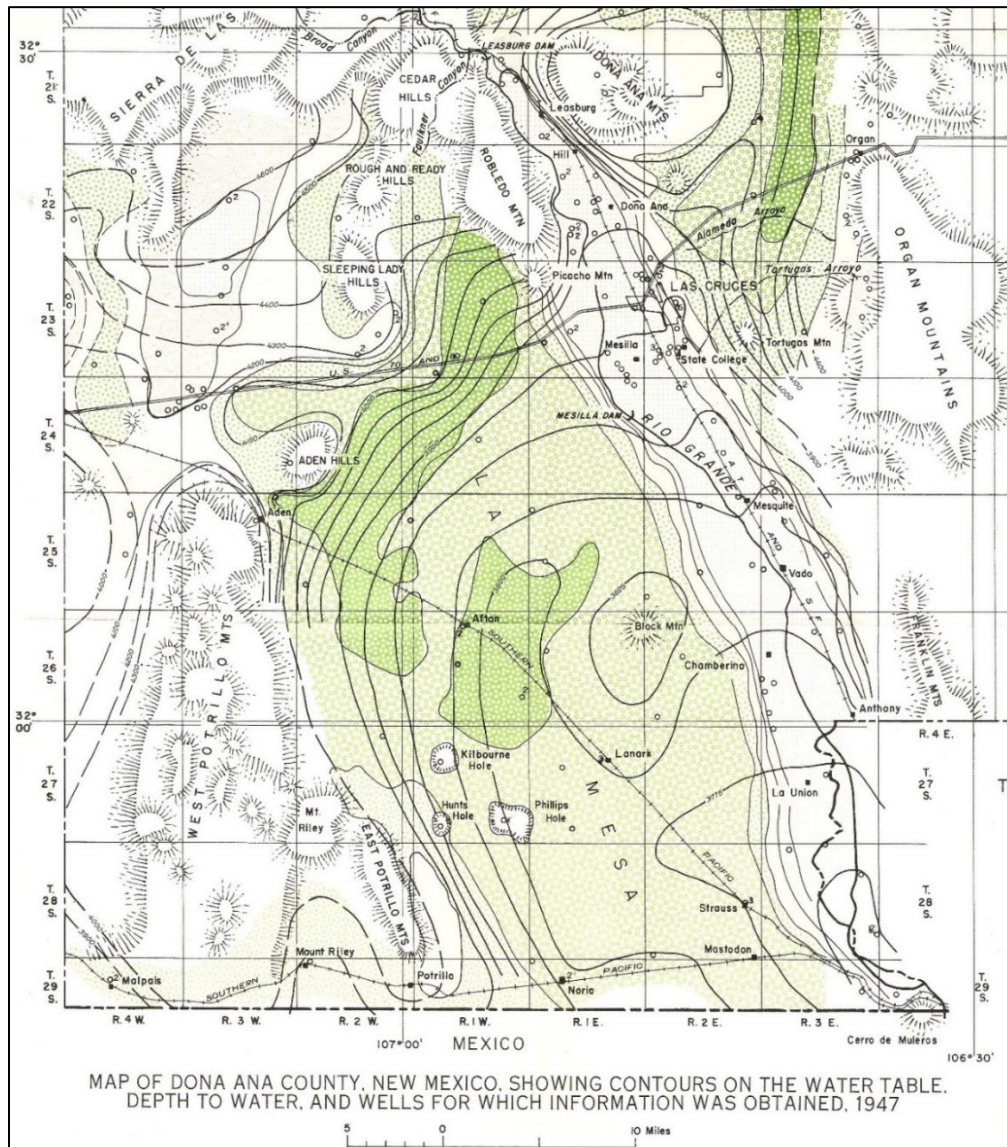
Figure 7-11 (facsimile copy of central and southern parts of Plate 1 in Conover 1954 [partial PL. 9A]). Map showing the approximate 1947 water-table altitude in central and southern Doña Ana County, with estimated depths to water in the 300 to 400 ft and > 400 ft ranges shown, respectively, with light greenish yellow and green dotted patterns.
