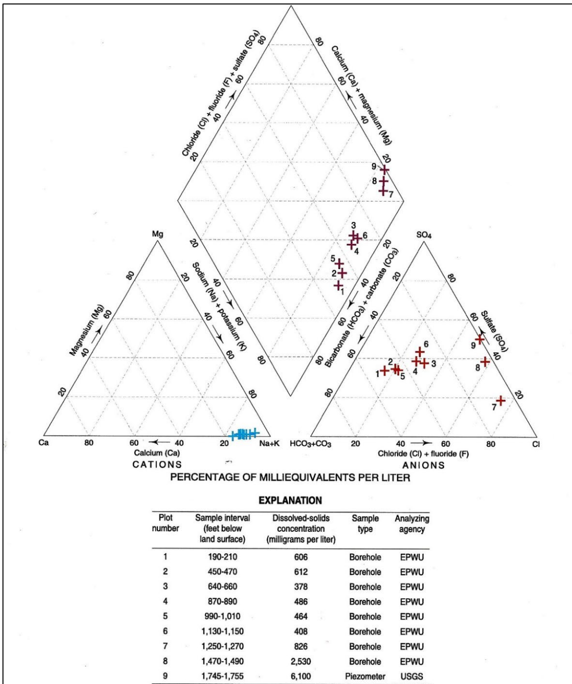
Figure 6-16 (Nickerson 2006, Fig. 4). Distribution of major constituents in groundwater-quality samples from selected depth intervals at the LMV-3 site (TBL. 1, no. 248). Sampled intervals by HSU and LFA: (1) 190-210 ft (58-61 m)–basal USF2 (LFA 3), (2) 450-470 ft (137-143 m)–upper MSF2 (LFA 3), (3) 640-660 ft (195-196 m)–lower MSF2 (LFA 3), (4) 870-890 ft (265-271 m)–MSF (LFA 4), (5) 990-1,010 ft (302-308 m)–basal MSF2 (LFA 3), (6) 1,130-1,150 ft (344-350 m)–upper LSF (LFA 4), (7) 1,250-1,270 ft (381-387 m)–upper LSF (LFA 4), (8) 1,470-1,490 ft (448-454 m)–LSF (LFA 9), and (9) 1,745-1,755 ft (532-535 m)–LSF (LFA 9). GW silica content (mg/L): (1) 43.6, (2) 44.7, (3) 44, (4) 44.6, (5) 43.8, (6) 30.1, (7) 22.5, (8) 29.5, and (9) 31.9 (cf. Nickerson 2006, Appendix Table 2, p. 22).
