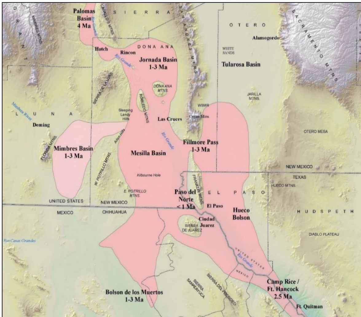
Figure 3-7 (Hawley et al. 2009, Fig. 9). Schematic depiction of the approximate area where fluvial and fluvial-deltaic deposits of the Ancestral Rio Grande (ARG) form the dominant Upper SFG basin-fill component. The primary distributary-channel network that spread out from an apex at the end of a trunk ARG channelbelt in the Palomas Basin northwest of Hatch is in dark pink. Million-yr (Ma) age ranges of major distributary channelbelts are based on geochronologic information available in 2008. The network terminated in fluvial-deltaic transition zones that bordered the paleo-Lake Cabeza de Vaca (LCDV) system of Strain (1966; cf. Part 3.7.2 ). The “Bolson de los Muertos” rift-basin complex of Chapin and Seager (1975) is located in the “Acuífero Conejos Médanos” section of the northern ZHGCM ( Figs. 1-10, 1-11, and 3-3 ).
