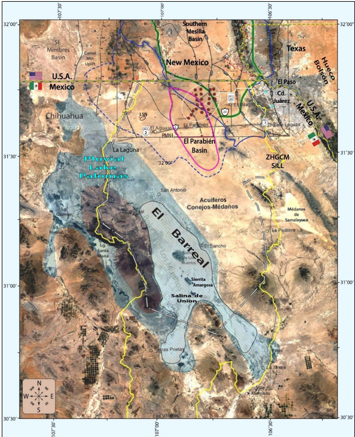
Figure 7-3 (page-size PL. 11 ). Index map for major GW-management and geohydrologic units in Mexico and the United States that is compiled on a 2018 Google Earth® image-base. The El Parabién and southern Mesilla GW Basins are outlined in violet and green, and the Study Area border is in black. The black-dashed and white line is the “delineación oficial” of the “Acuífero Conejos-Médanos,” and the larger “Zona Hidrogeológica de Conejos Médanos (ZHGCM)” is bounded with a solid yellow line (INEGI 2012).
