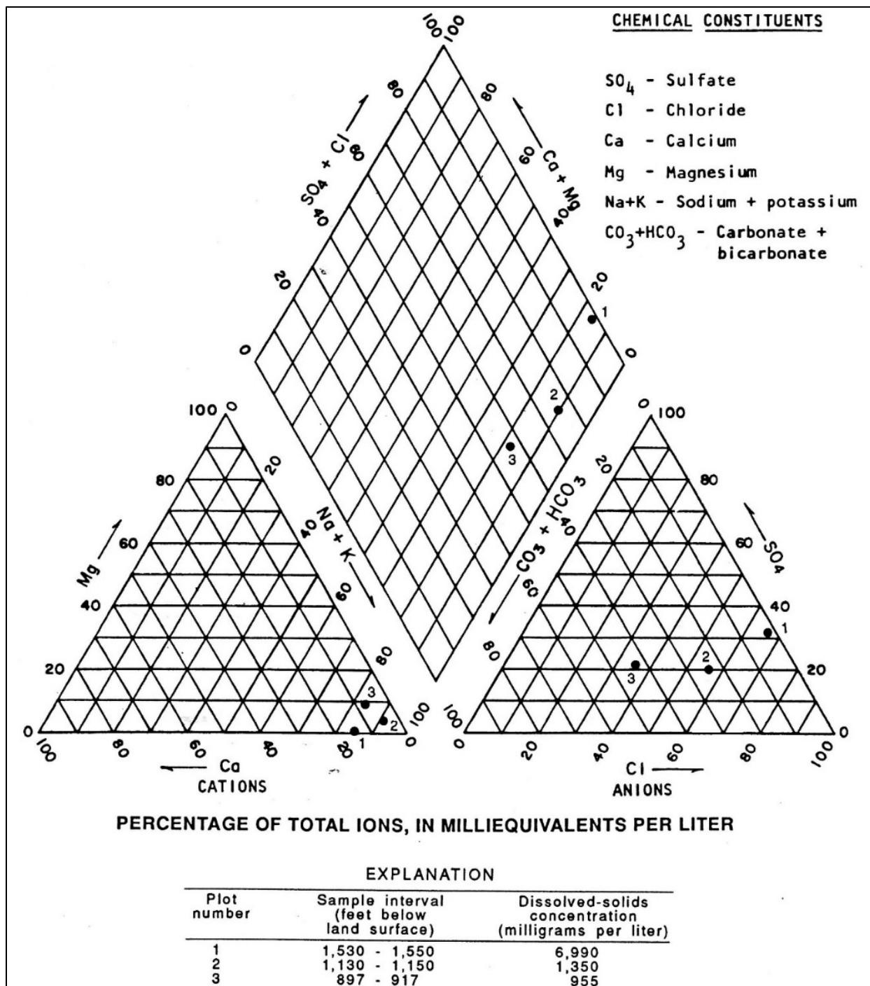
Figure 6-5 (Nickerson and Myers 1993, p. 62, Fig. 40). Chemical analyses of water from selected depth intervals in the Lanark test hole (USGS-EPWU, TBL. 1, no. 236). Samples from: (1) uppermost part of the Lanark igneous-intrusive complex (PLS. 5i, 5q, and 8B: TmLC-Tmi/Tlvs), (2) upper part of HSU-LSF (LFA-7), and (3) HSU-MSF (LFA 3). Sample temperature and silica content (Celsius and mg/L): (1) 42.5° and 63, (2) 35° and 52, and (3) 31.5° and 67 (cf. Hawley and Lozinsky 1992, Tbl. 4a, Nickerson and Myers 1993, Tbl. 2).
