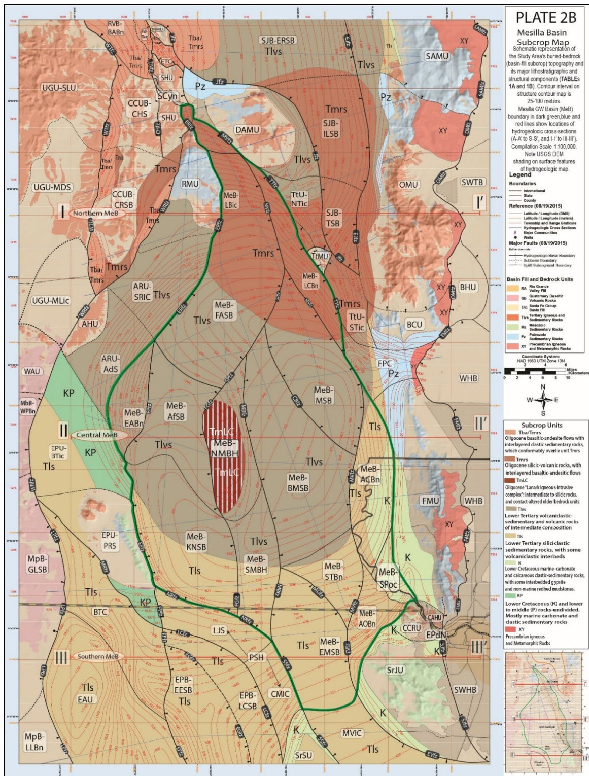
Figure H1-19 (page-size Rpt. PL. 2B ). Schematic depiction of basin-fill subcrop topography, and primary lithostratigraphic and structural components in the Study Area, with explanation on Table H1-10 . W-E red lines show locations of geologic cross-sections I-I' to III-III' on Figure H1-20 . Swanson Geoscience LLC compilation on Report PLATE 1 hydrogeologic-map base.
