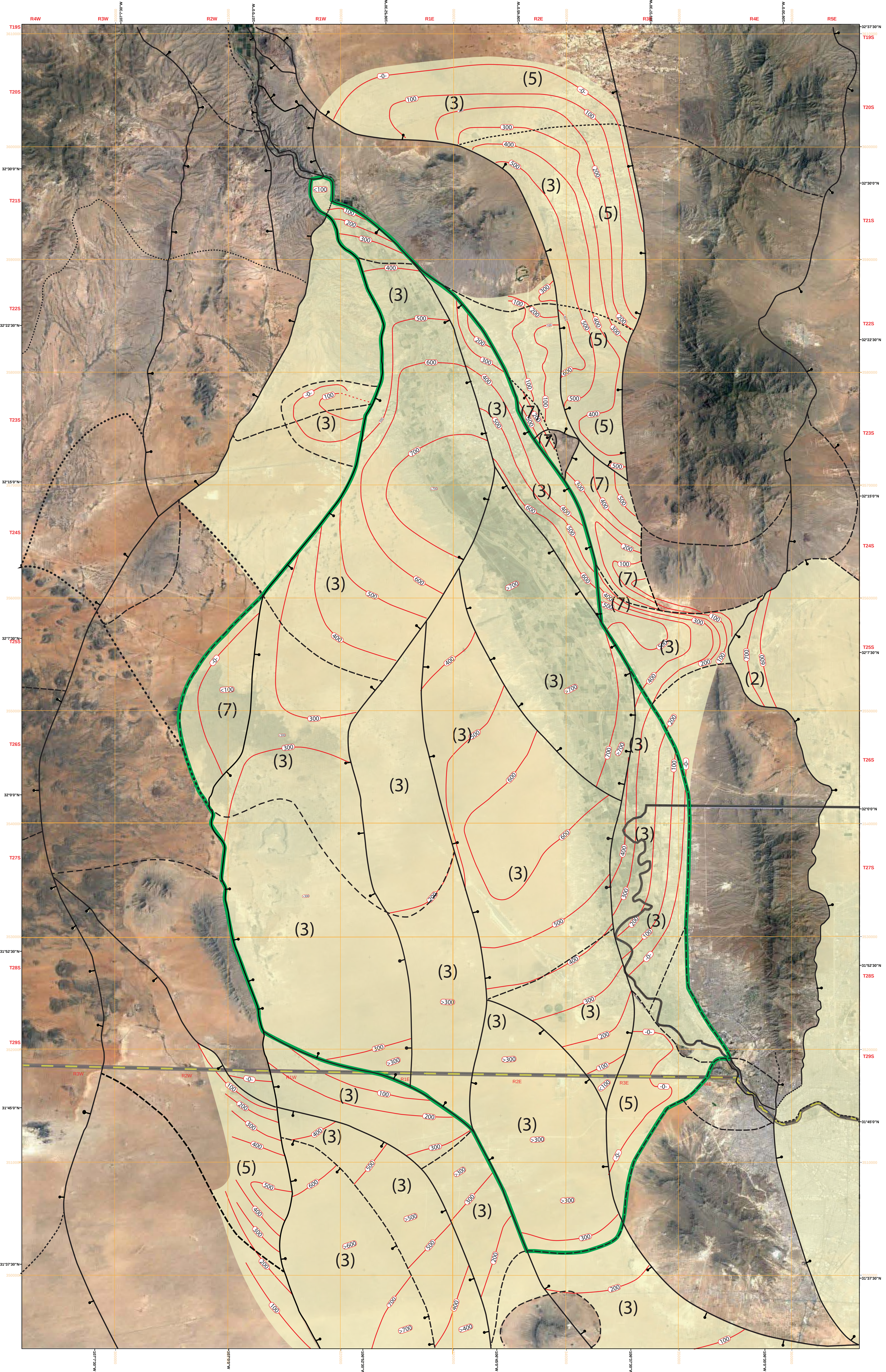
PLATE 7A Isopleth of Pre-development saturated Upper Santa Fe Group of the Mesilla Basin
