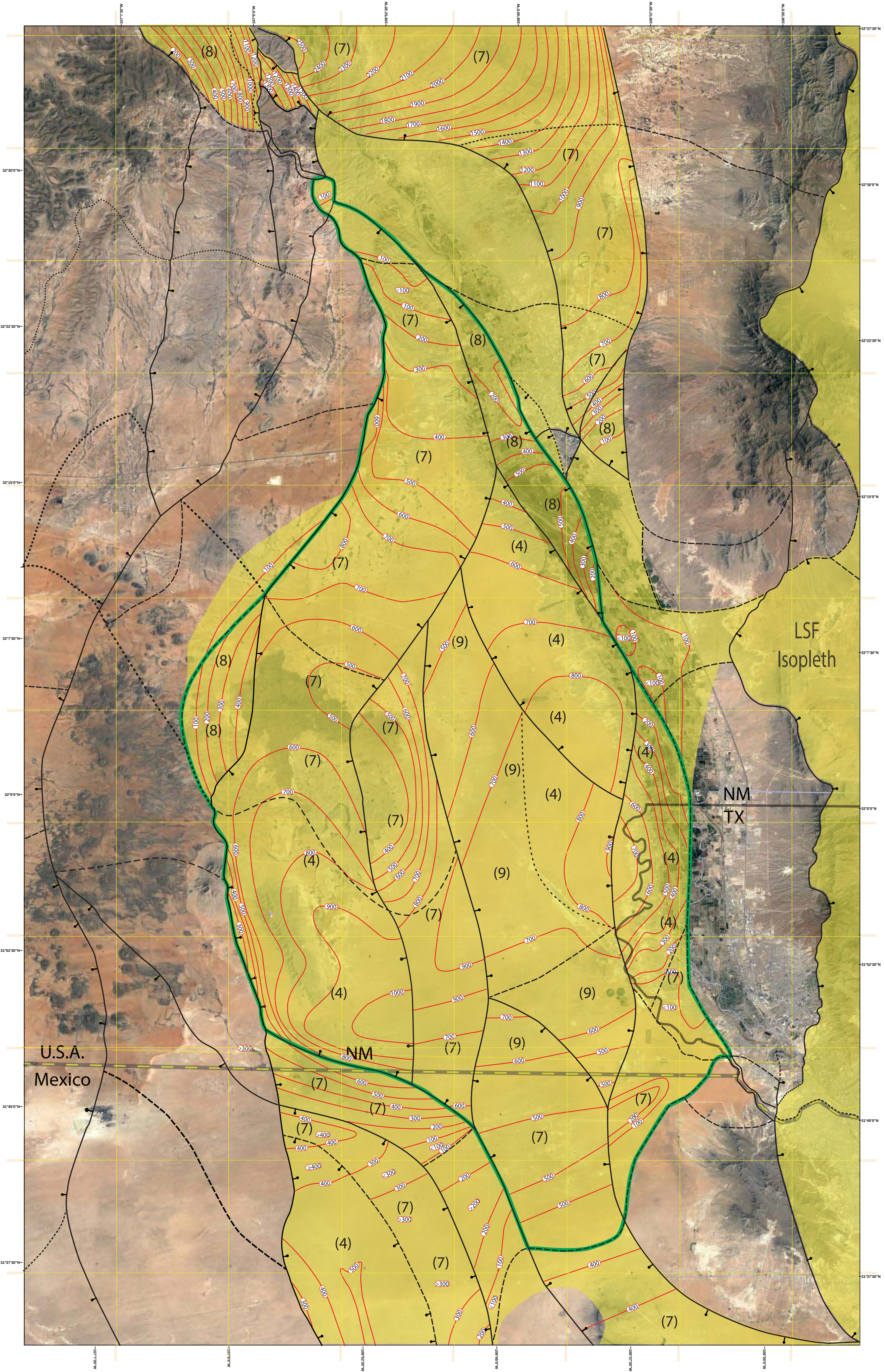
PLATE 7C Isopleth of Lower Santa Fe Group of the Mesilla Basin
