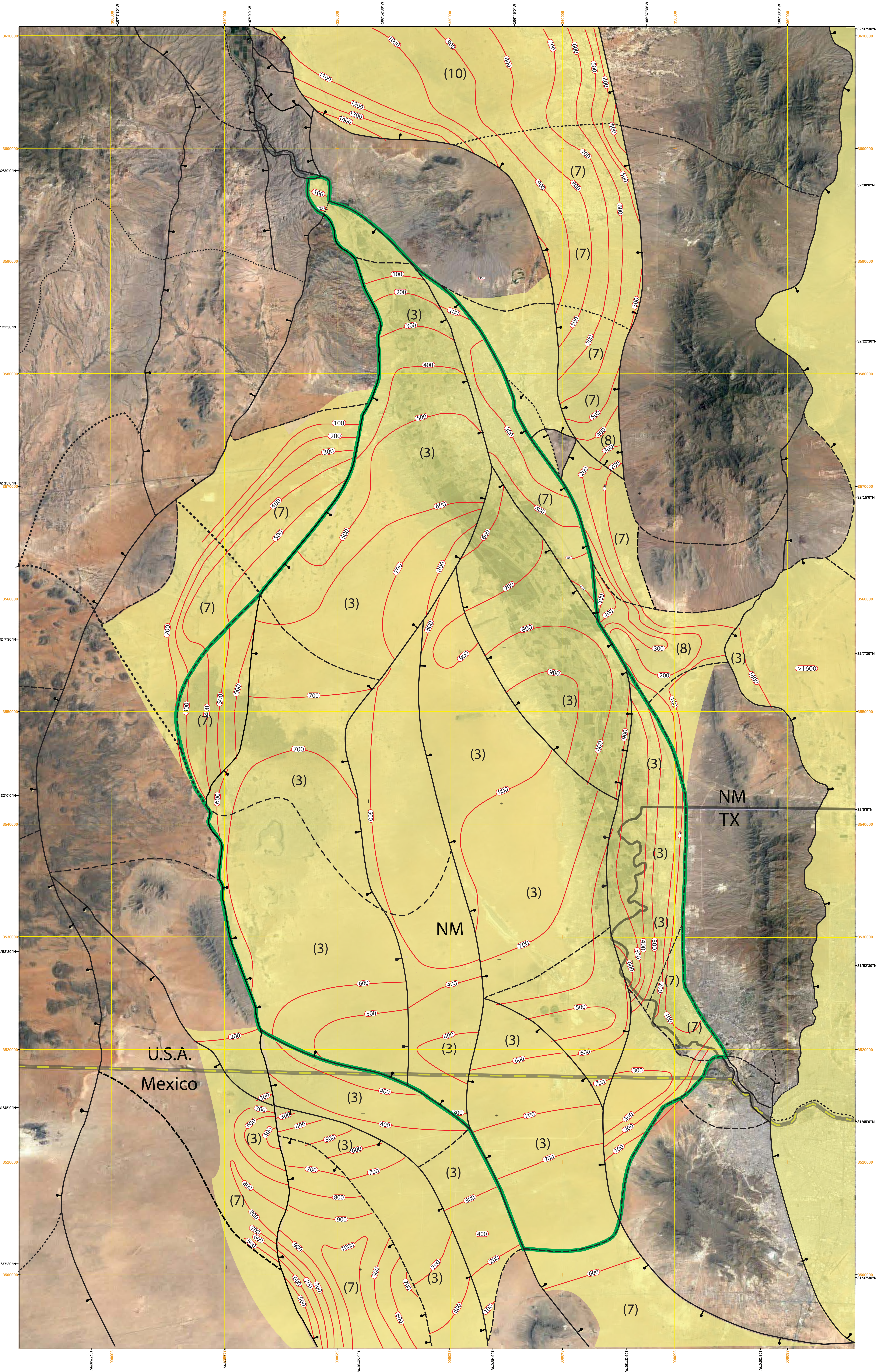
PLATE 7B Isopleth of Middle Santa Fe Group of the Mesilla Basin
