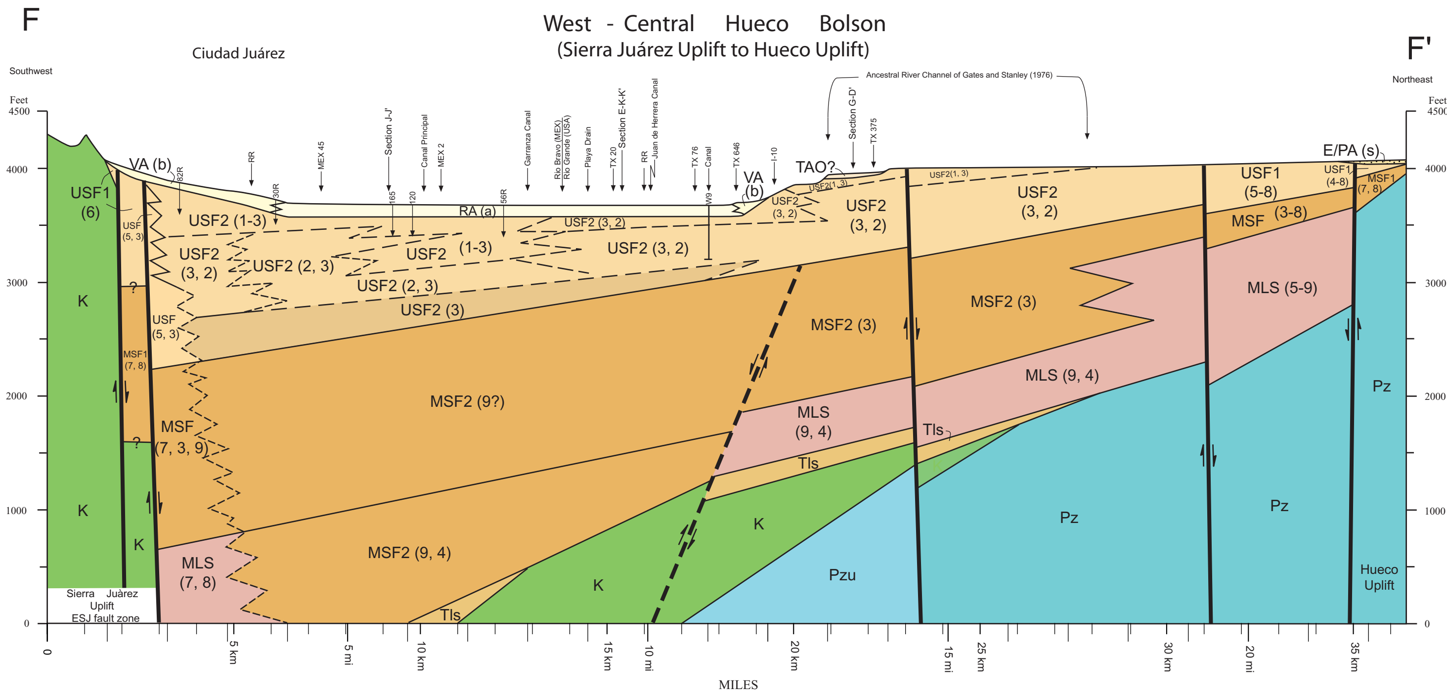
Schematic Hydrogeologic Section -- F-F' - from Sierra Juárez to Hueco uplift, across central Ciudad Juárez area of western Hueco Bolson
