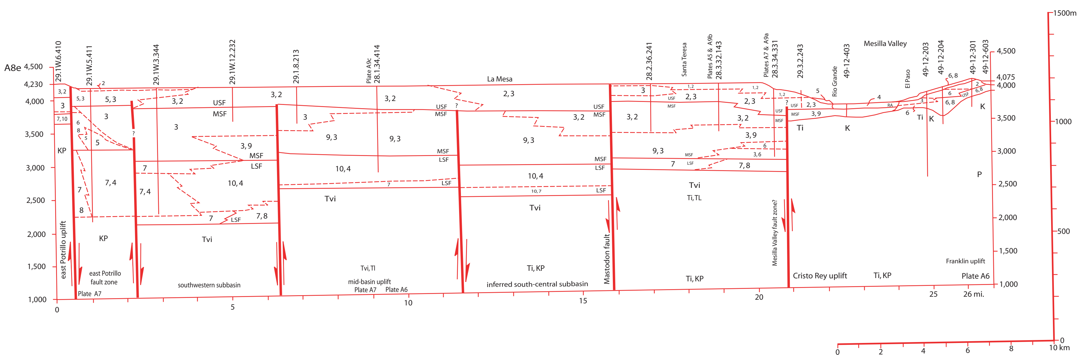
Plate A8. Hydrogeologic Sections of the Mesilla Basin, Las Cruces to El Paso area, showing inferred distribution of major hydrostratigraphic and lithofacies units, and fault zones
