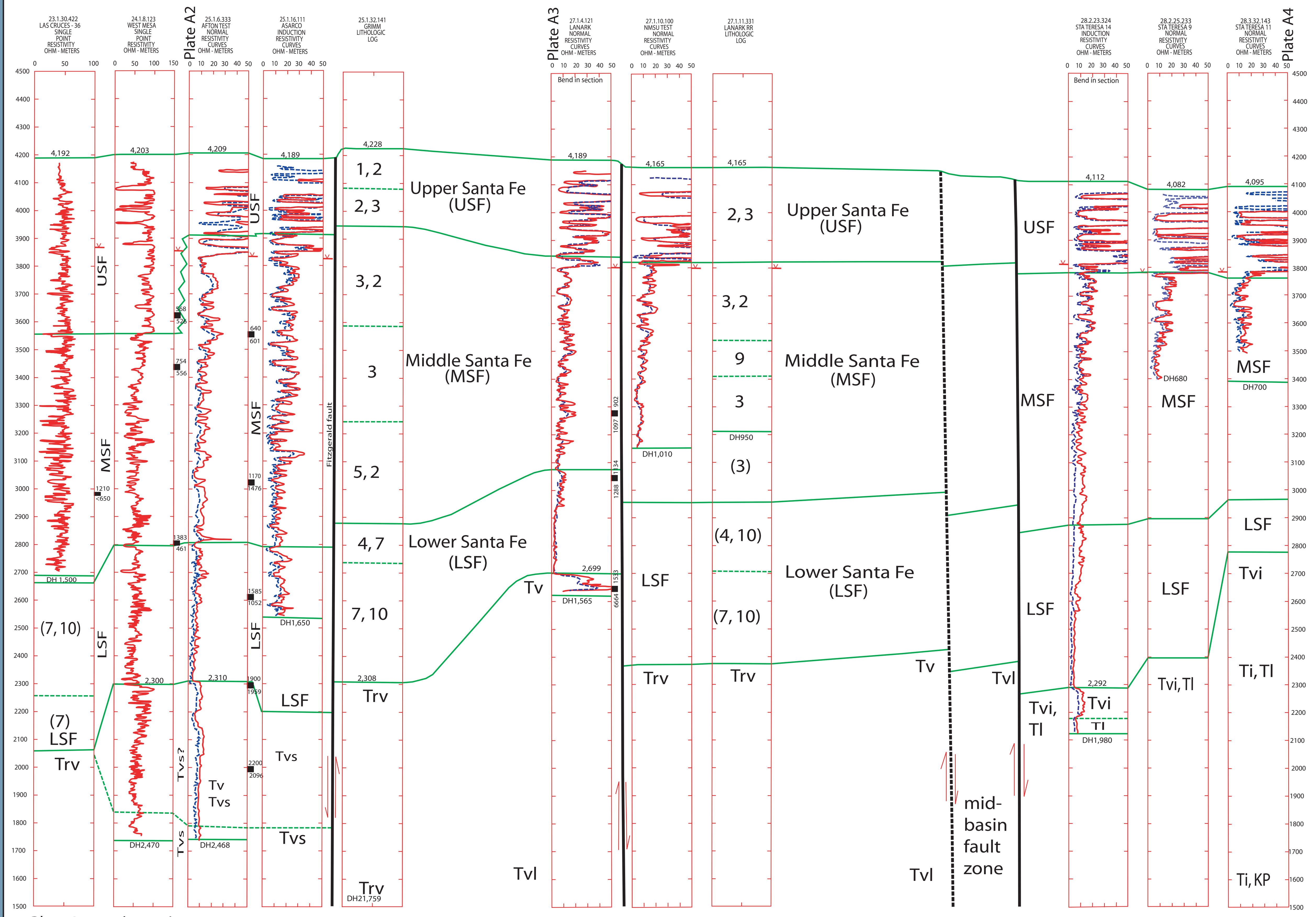
Plate A5. Hydrogeologic section Las Cruces to Santa Teresa, with borehole geophysical data.
