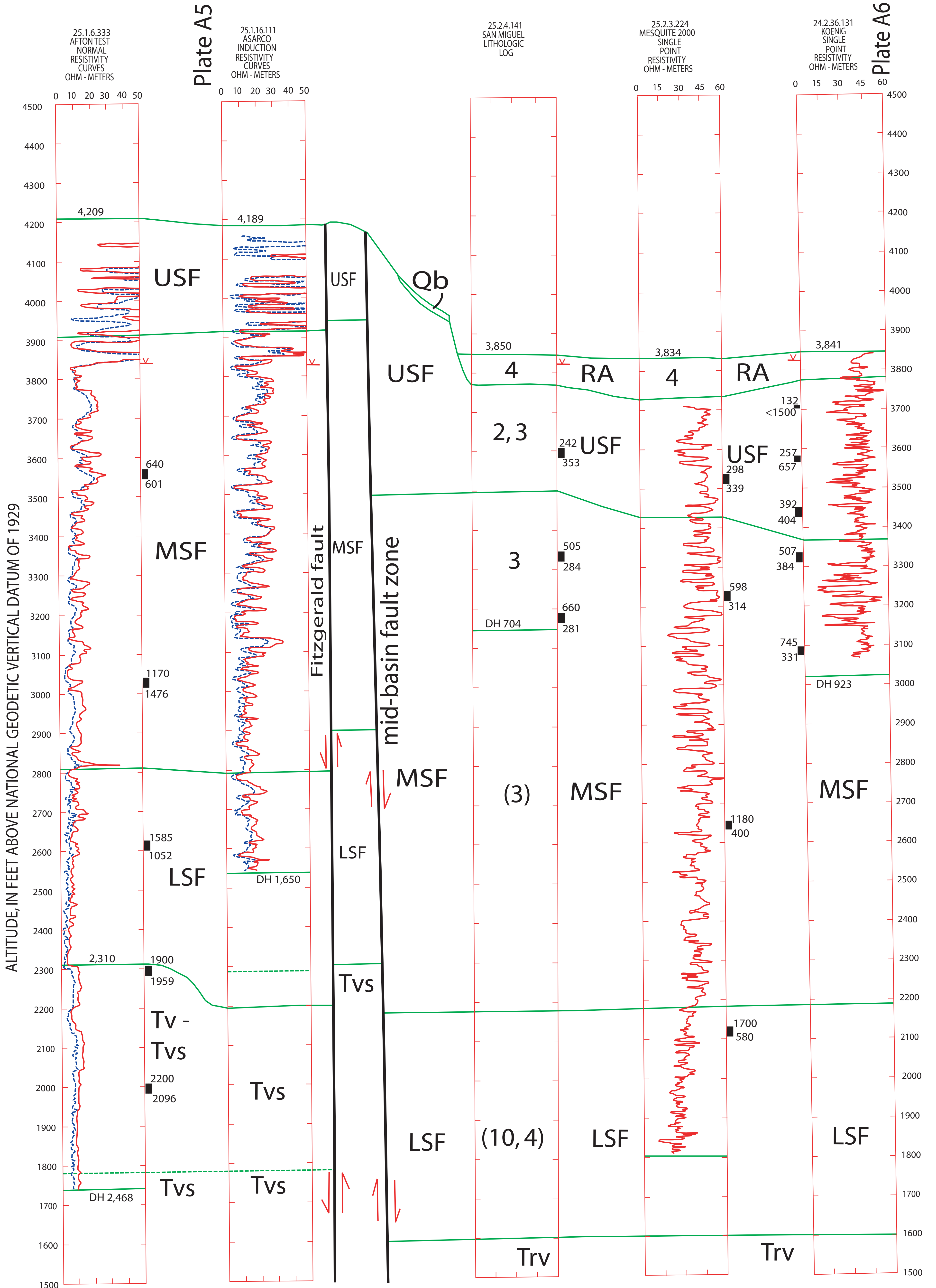
Plate A2. Hydrogeologic section Afton to Mesquite, with borehole geophysical data.
