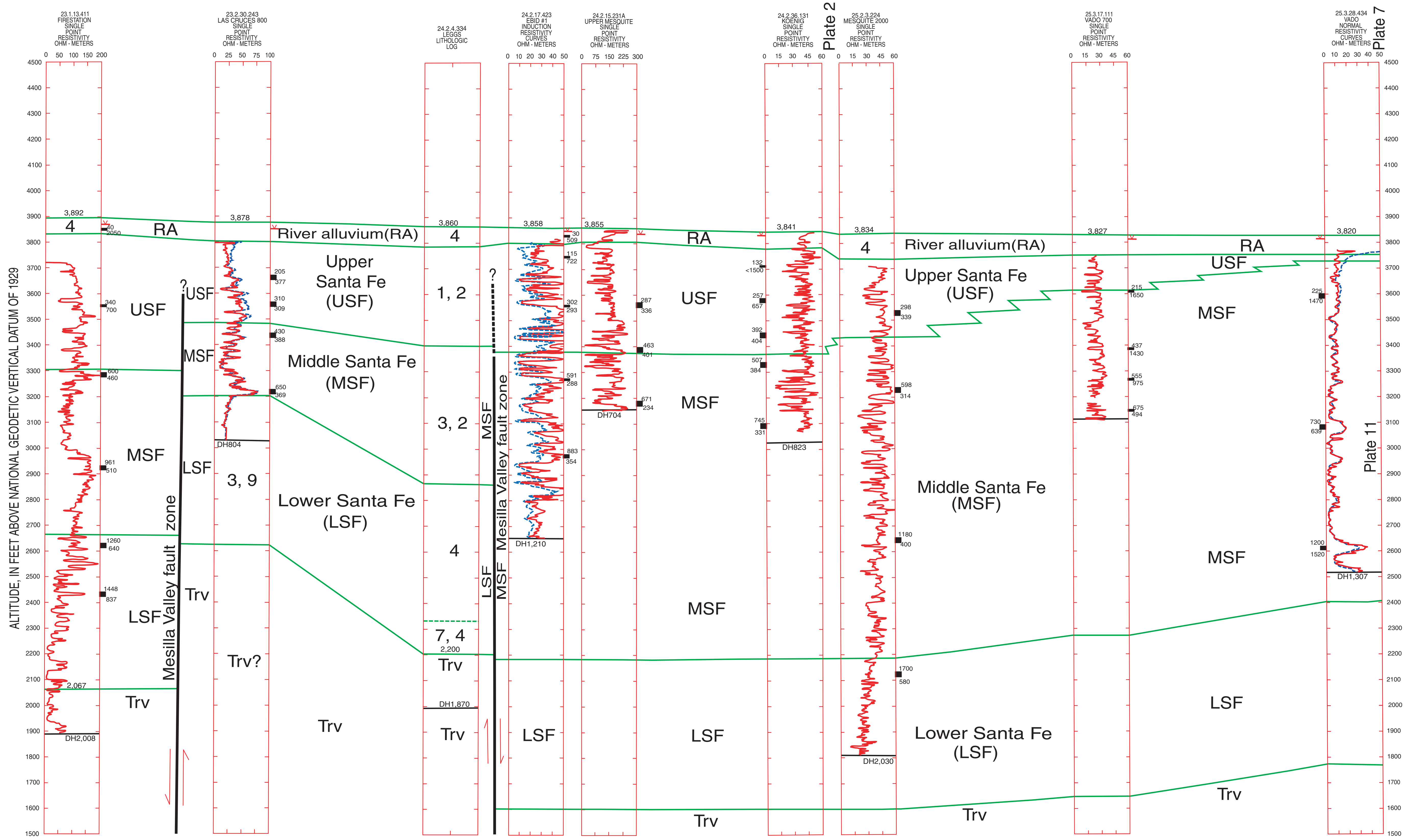
Plate 6. Hydrogeologic section Las Cruces Firestation to Vado, with borehole geophysical data.
