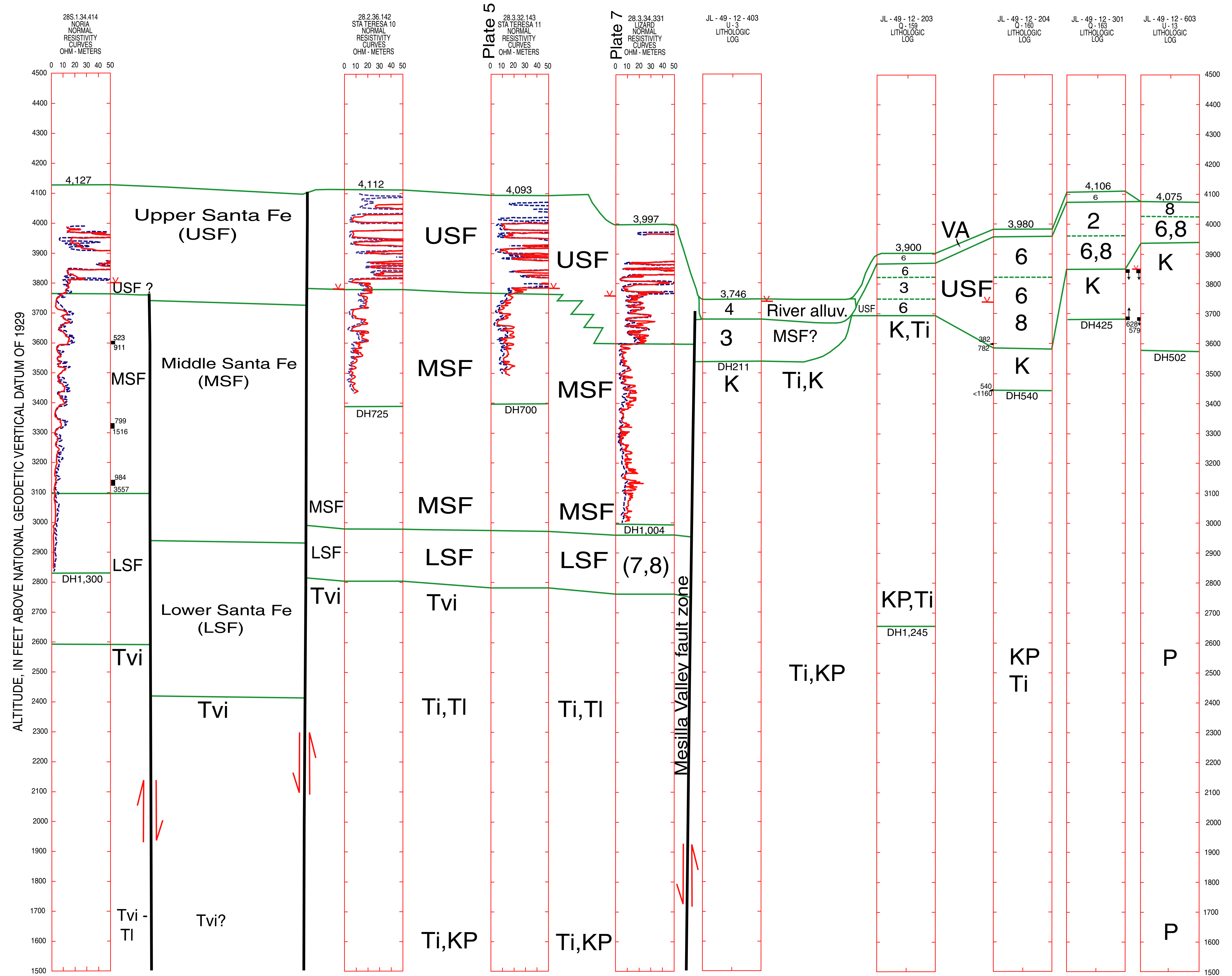
Plate 4e. Hydrogeologic section Noria Test to Mesa Boulevard, with borehole geophysical data.
