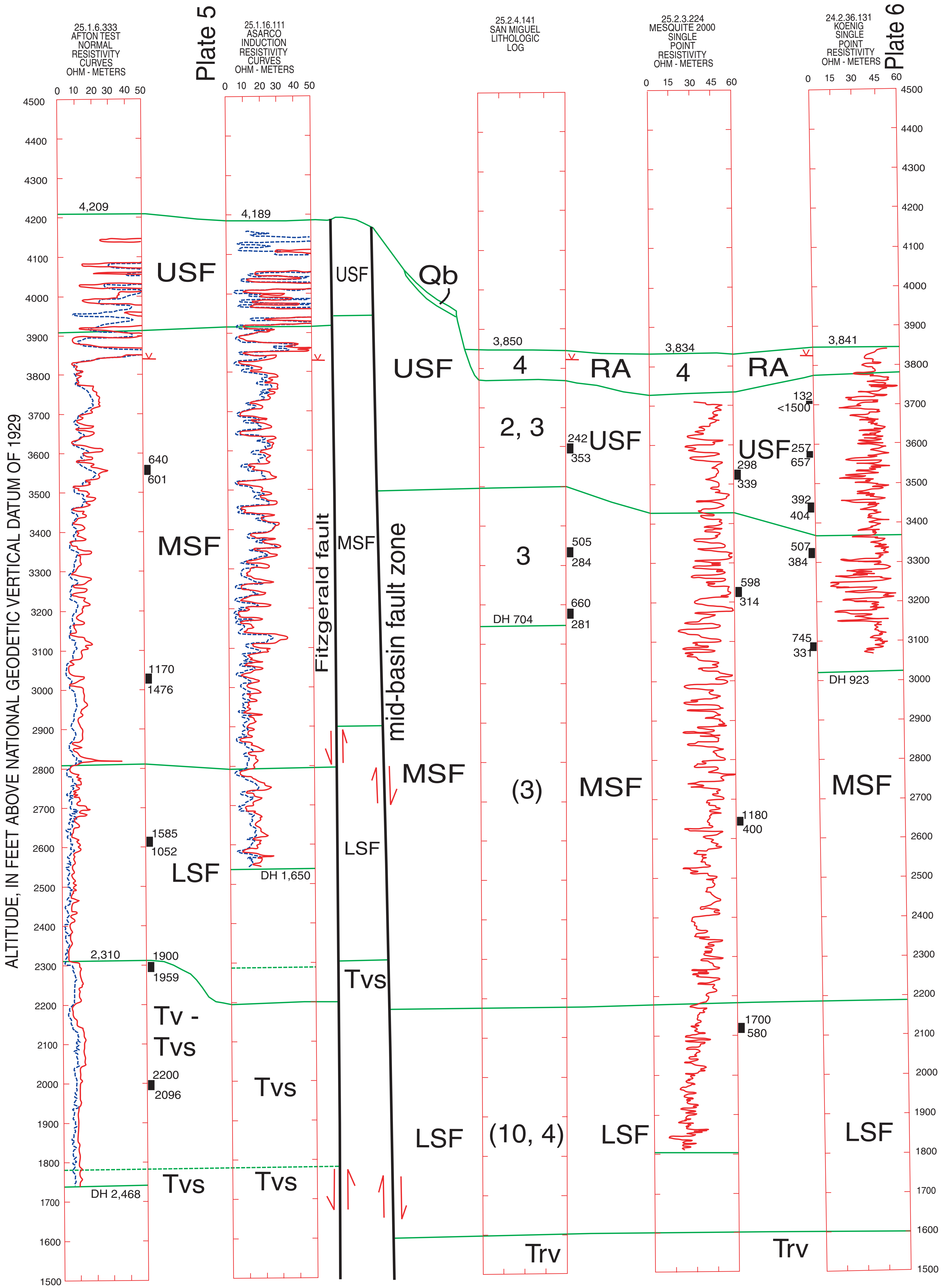
Plate 2. Hydrogeologic section Afton to Mesquite, with borehole geophysical data.
