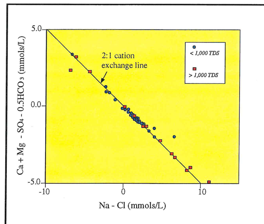
Figure 3.20. (Ca + Mg - \text{SO}_4 - 0.5\text{HCO}_3^- ) vs (Na - Cl) plot, group 3 and group 4 ground waters (source of data, Texas Water Development Board; Comision Nacional Del Agua; Instituto Nacional de Estadistica, Geografia e Informatica).
