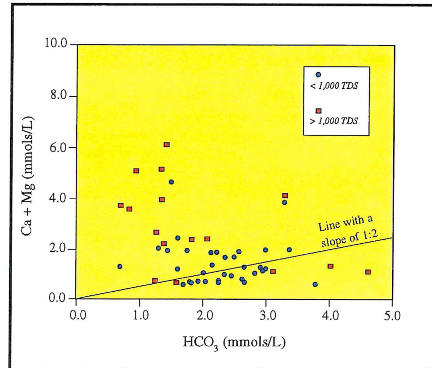
Figure 3.18. (Ca + Mg) vs \text{HCO}_3^- plot, group 3 and group 4 ground waters (source of data, Texas Water Development Board; Comision Nacional Del Agua; Instituto Nacional de Estadistica, Geografia e Informatica).
