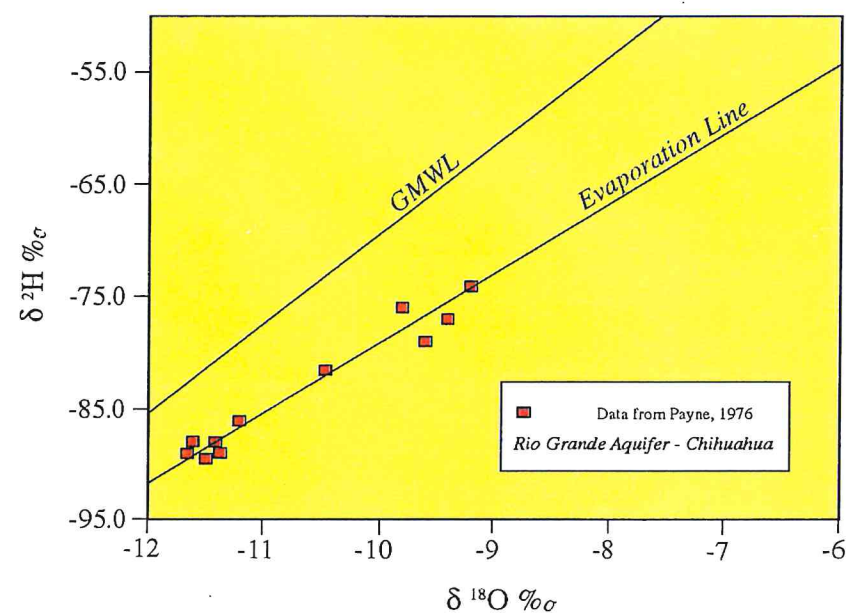
Figure 5.17. Binary plot of \delta^2\text{H} versus \delta^{18}\text{O} values for Rio Grande aquifer waters in the Mexican part of the alluvial aquifer. Stable hydrogen and oxygen isotope ratios in ground waters plot along the evaporation line, indicating evaporative enrichment of water, probably during irrigation (source of data, Payne, 1976).
