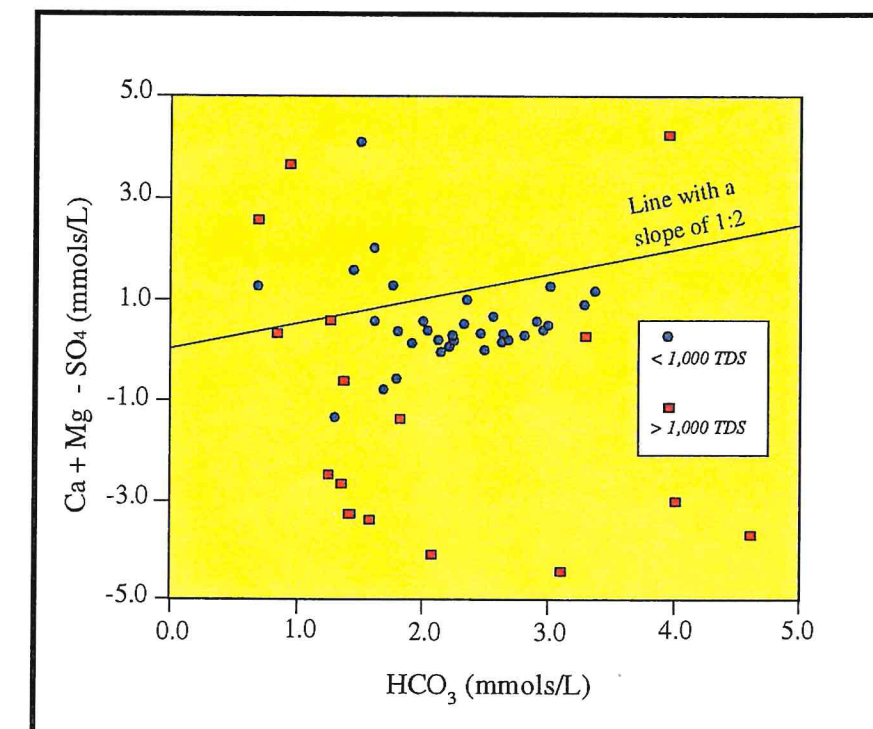
Figure 3.19. (Ca + Mg - \text{SO}_4 ) vs \text{HCO}_3^- plot, group 3 and group 4 ground waters (source of data, Texas Water Development Board; Comision Nacional Del Agua; Instituto Nacional de Estadistica, Geografia e Informatica).
