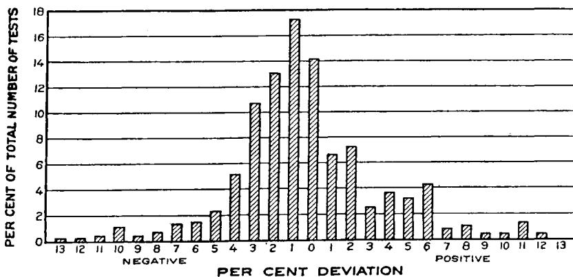
Figure 9.—Comparison in percentage of computed with observed submerged-flow discharge through experimental flumes.
