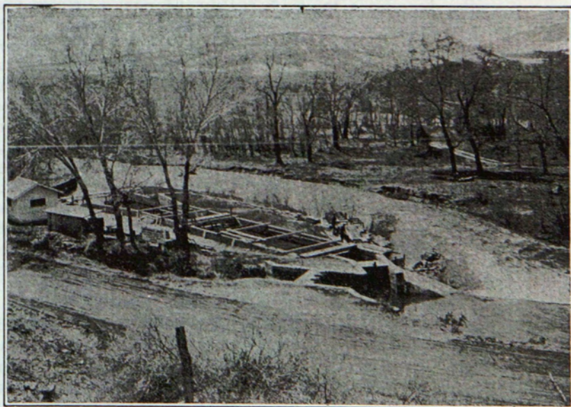
Figure 2.—Irrigation hydraulic laboratory at Bellvue, Colo.
