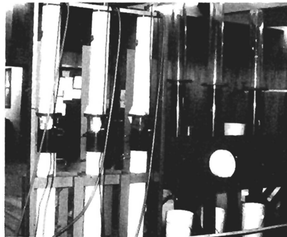
Figure 3. Laboratory scale series intermittent sand filters at the Utah Water Research Laboratory.
