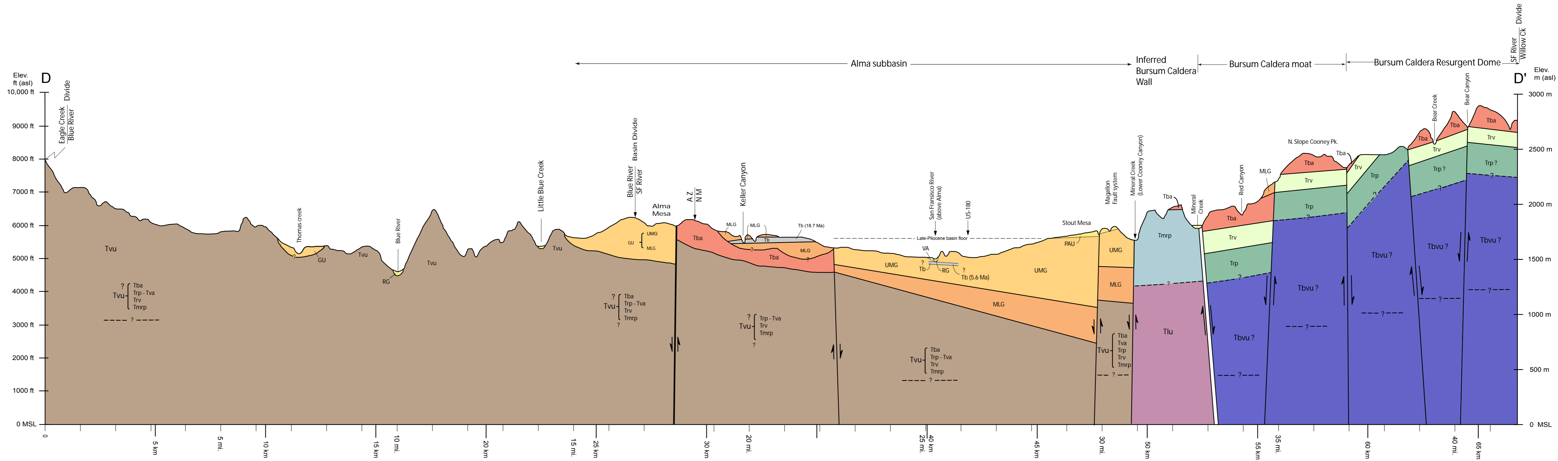
Plate 2d. Schematic Hydrogeologic Section D - D' Blue River basin (AZ), Alma subbasin (graben), and San Francisco River Valley above Alma: Blue River-Eagle Creek divide (near Rose Peak) to Mineral Creek-Willow Creek (upper Gila) divide in Mogollon Mountains (western Bursum caldera) Vertical Exaggeration: 5X June, 2010 J.W. Hawley, B.J. Creel, BVN. P. Kambhammettu
