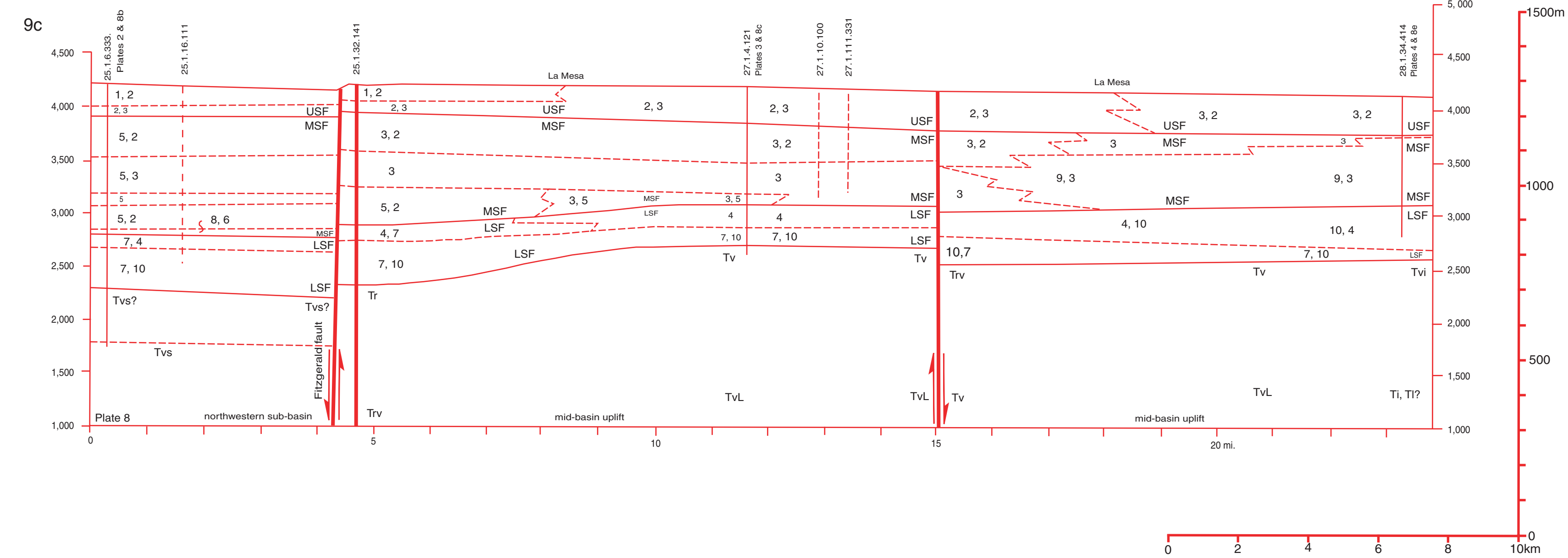
Plate 9 Hydrogeologic Sections of the Mesilla Valley and west central Mesilla Basin areas, showing inferred distribution of major hydrostratigraphic and lithofacies units, and fault zones
