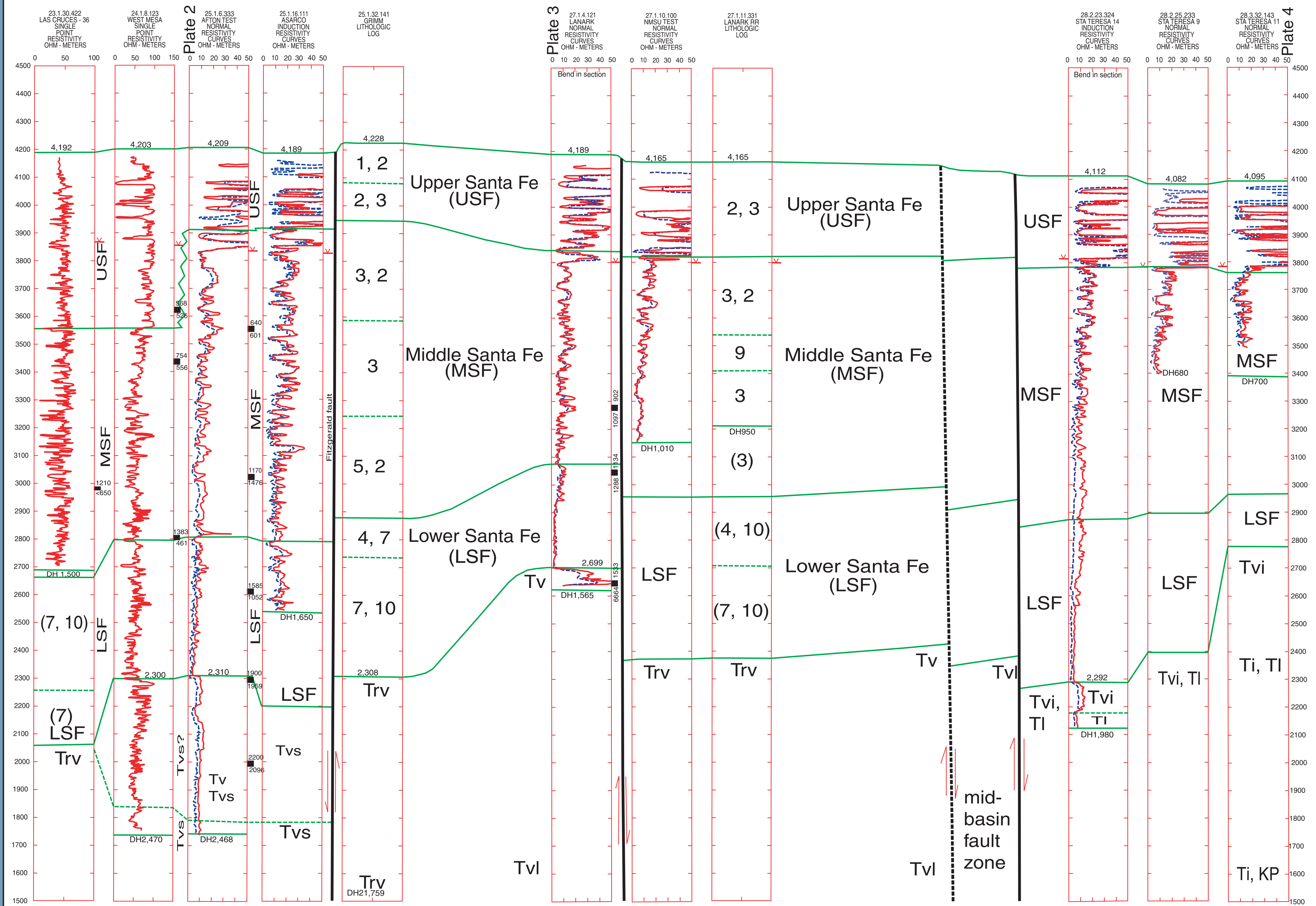
Plate 5. Hydrogeologic section Las Cruces to Santa Teresa, with borehole geophysical data.
